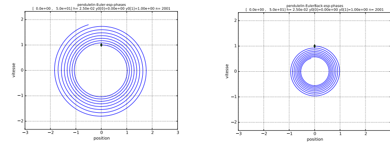
FIGURE 4 – Euler progressive : instable, amplification
